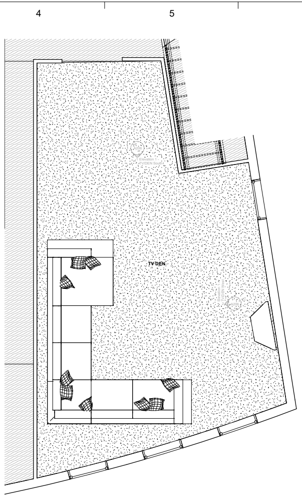
② 01-Ground Level Finish - Enlarge 1 1/2" = 1'-0"
